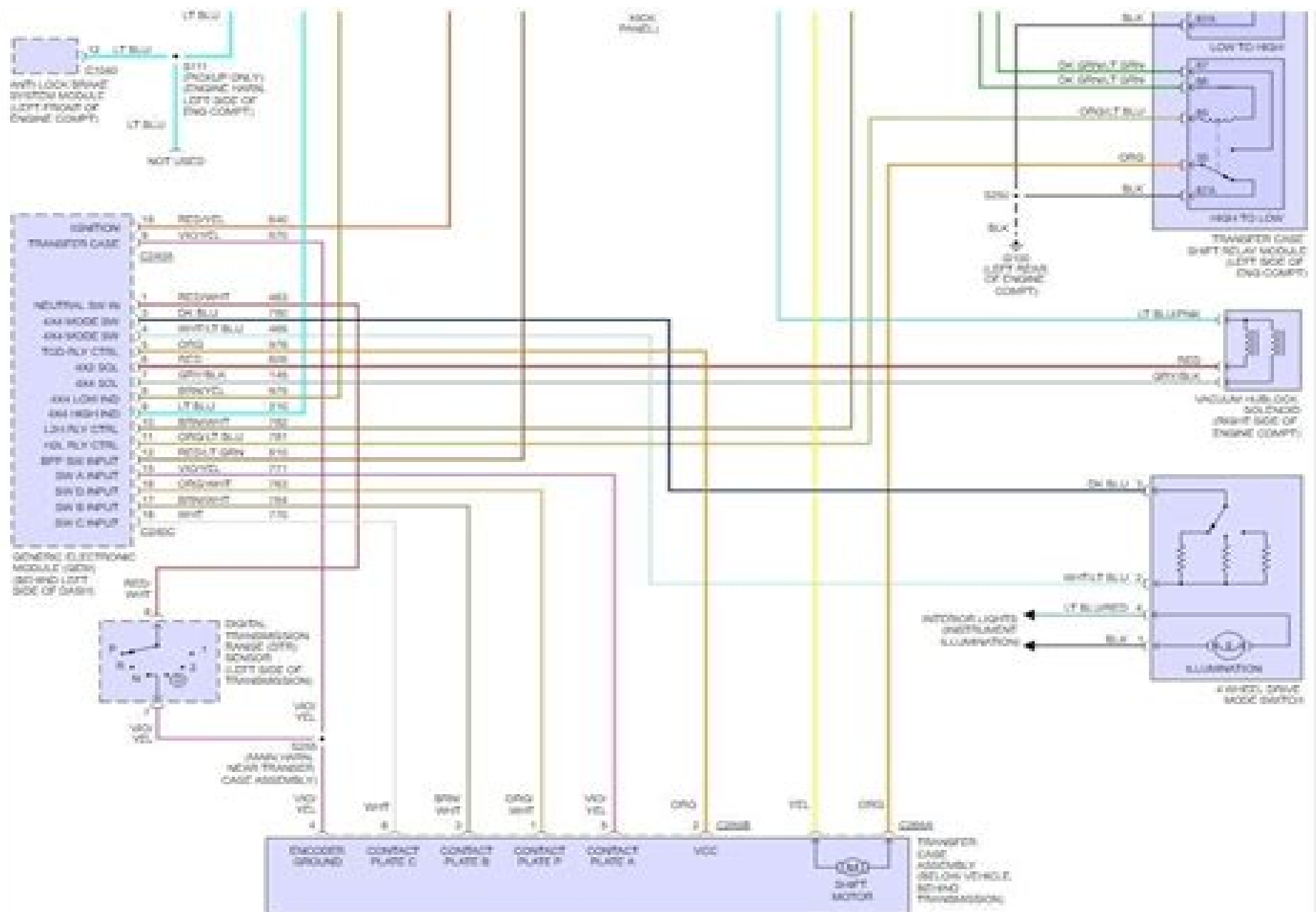
Fig 1: 4WD Circuit
