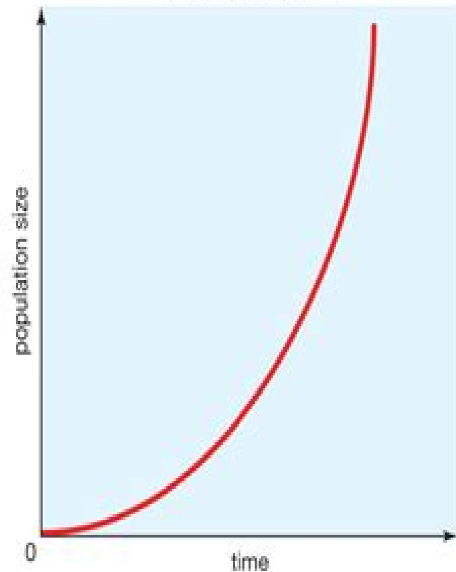
exponential growth
