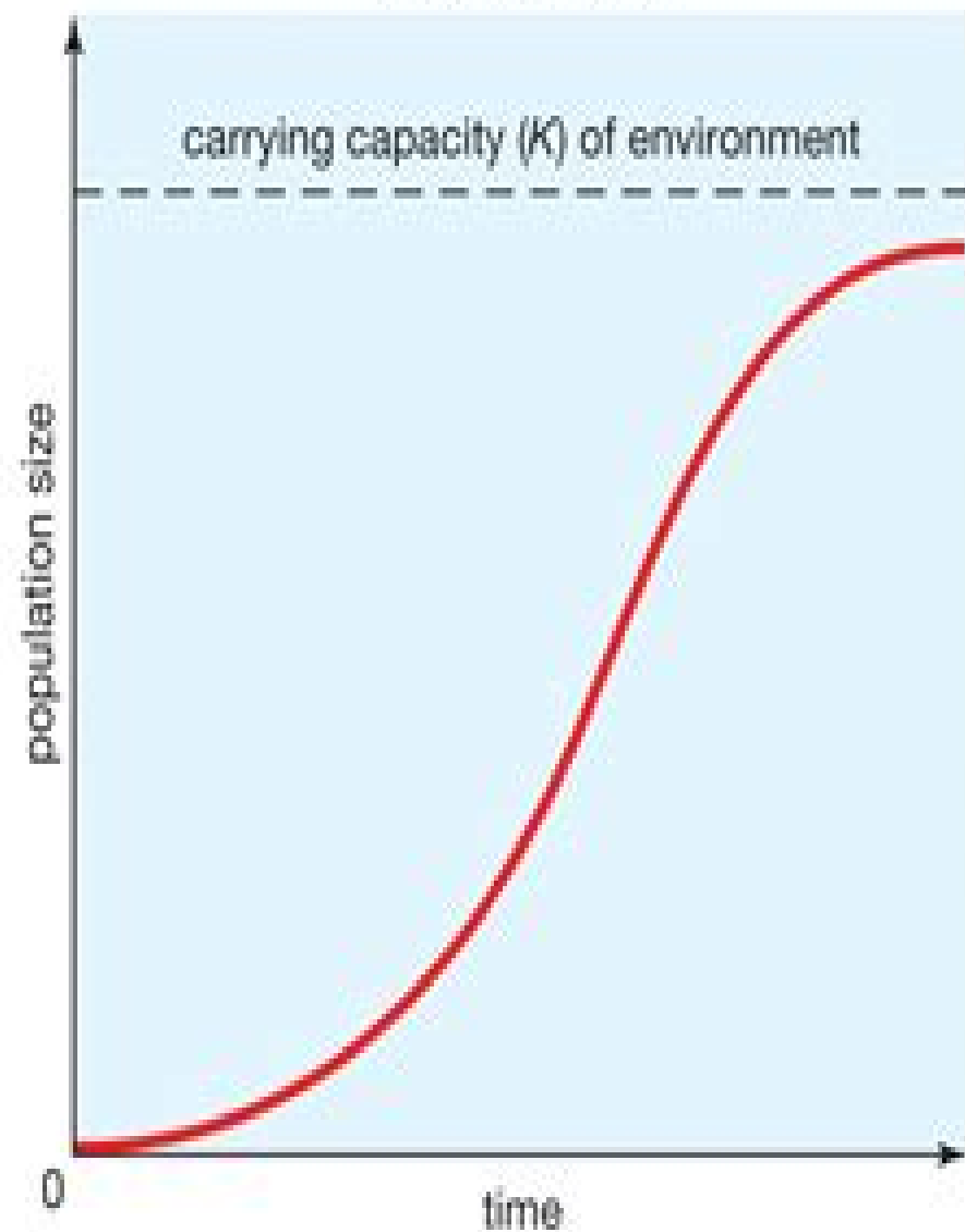
logistic growth
