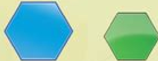
Similar Hexagons
