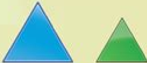
Similar Triangles
