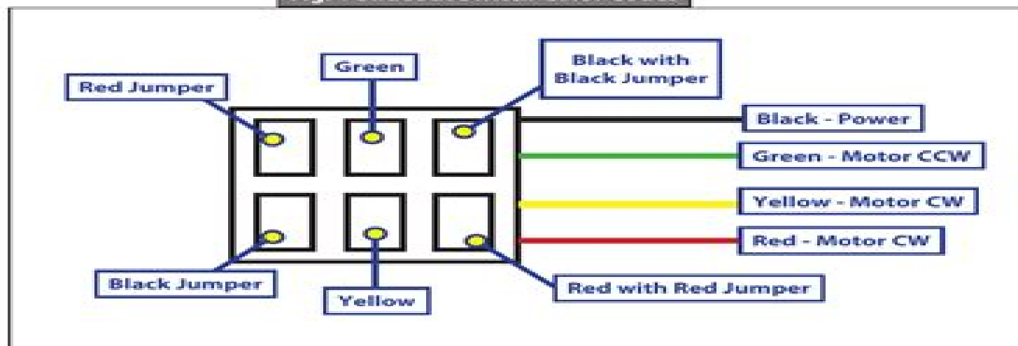
Fig. 1 Slideout Switch Color Codes
