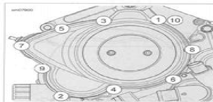
Figure 4-34. Tightening Sequence
