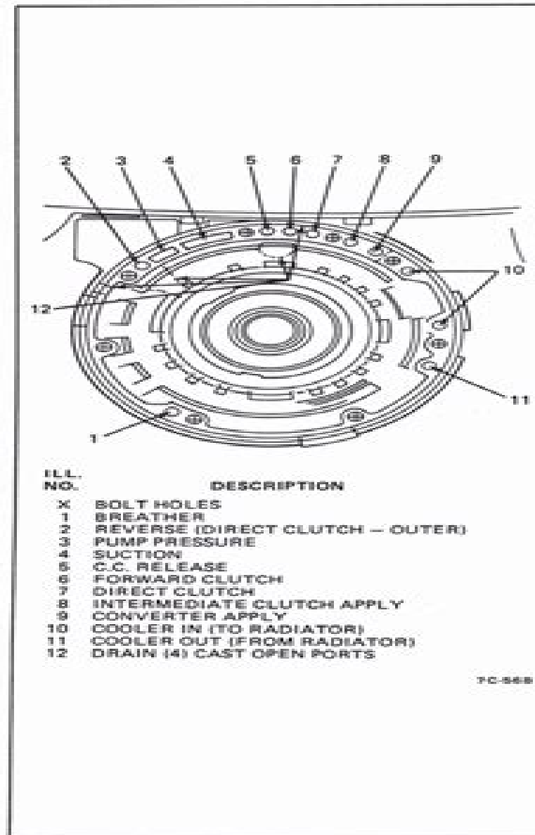
Figure 350C-10 Identification of Case to Pump Oil Passages
