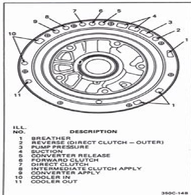
Figure 350C-9 Identification of Pump Rear Face Oil Passages
