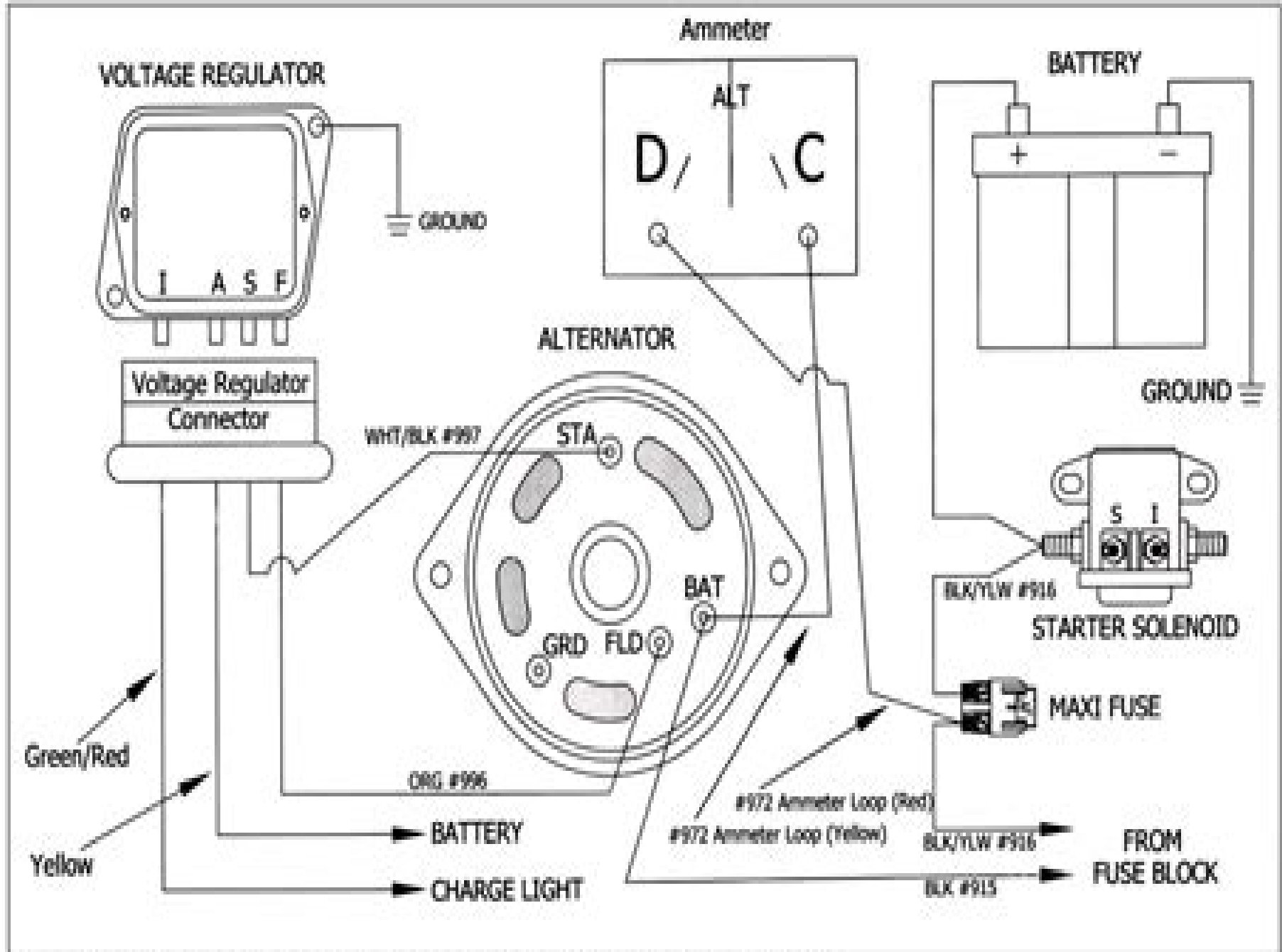
Figure 7-7 Alternator/Regulator/Solenoid Connections
