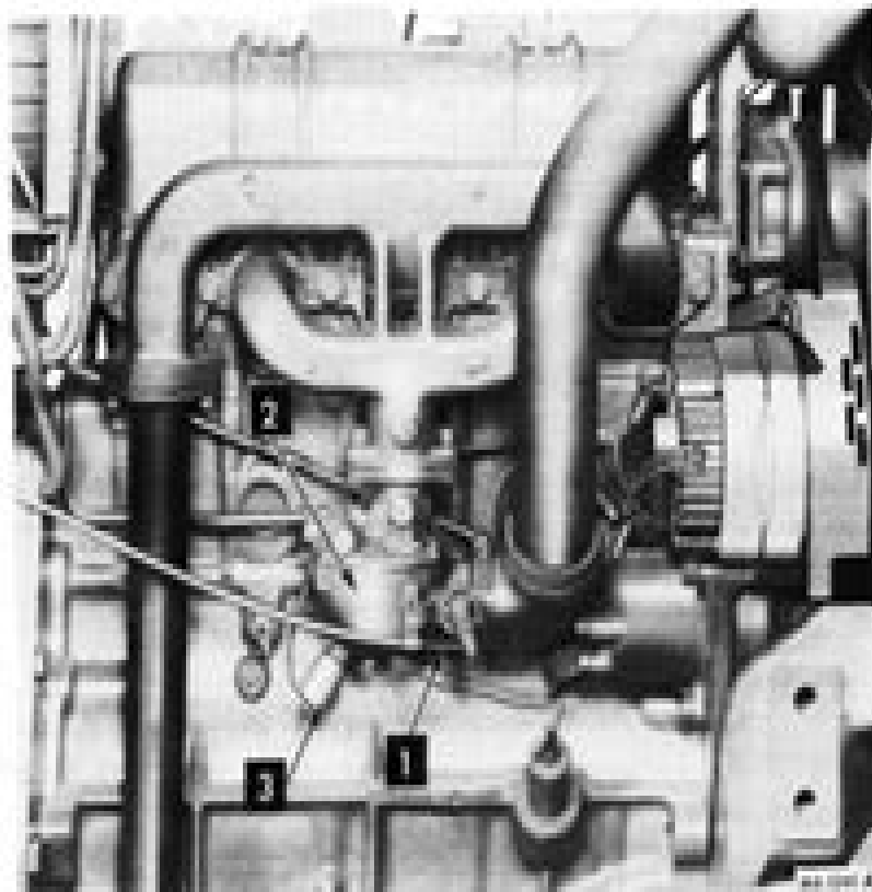
1 - Choke control wire 2 - Carburetor
