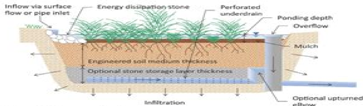
Figure 1. Cross-section view.
