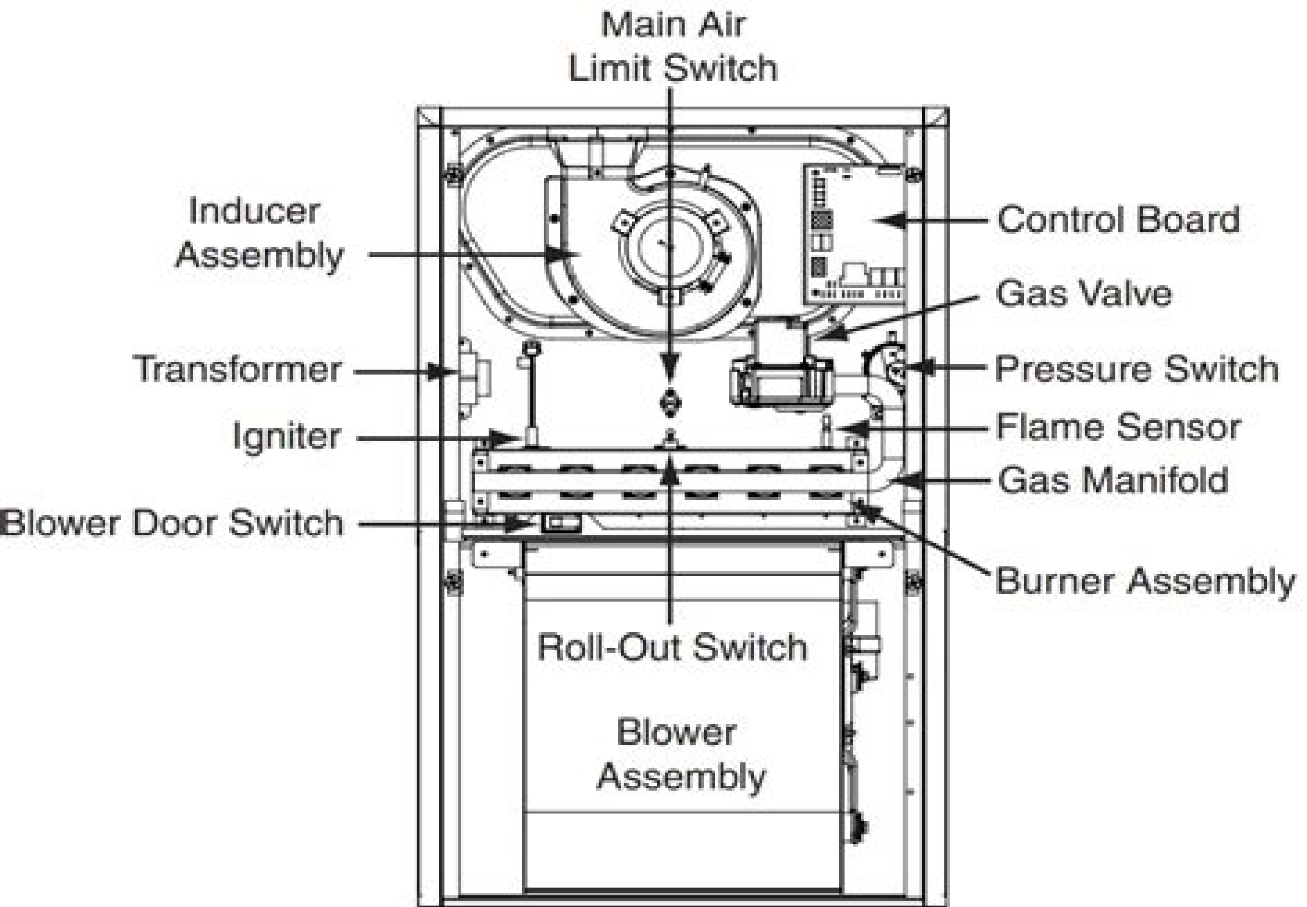
Upflow/Horizontal Gas Furnace
