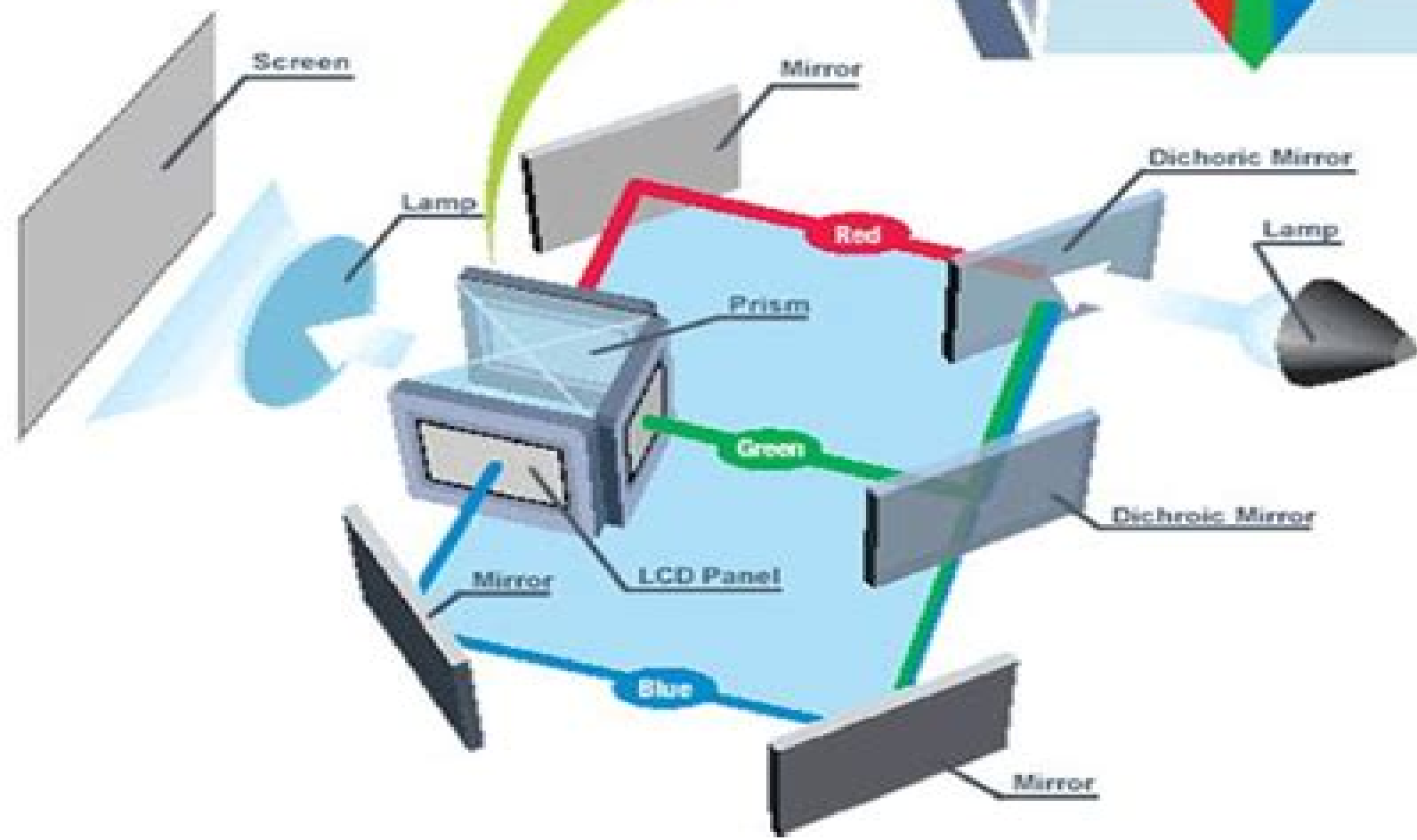
The Path of Light Through A 3LCD Projector
