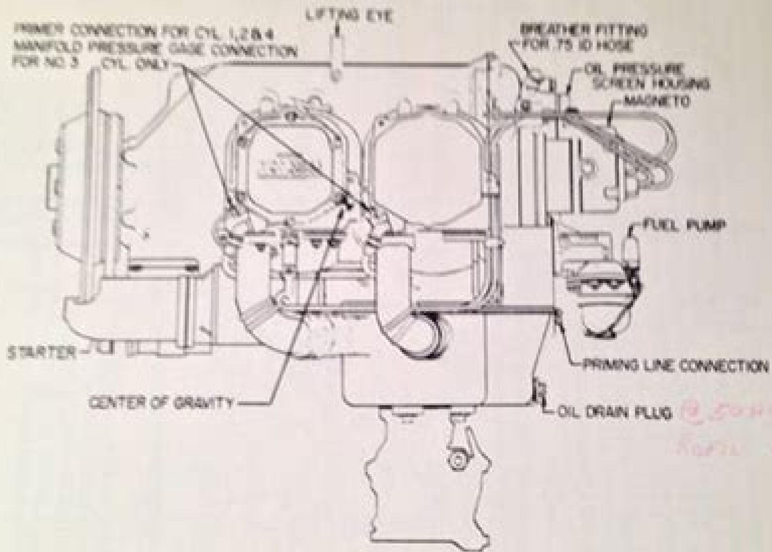
Installation Drawing - Left Side View
