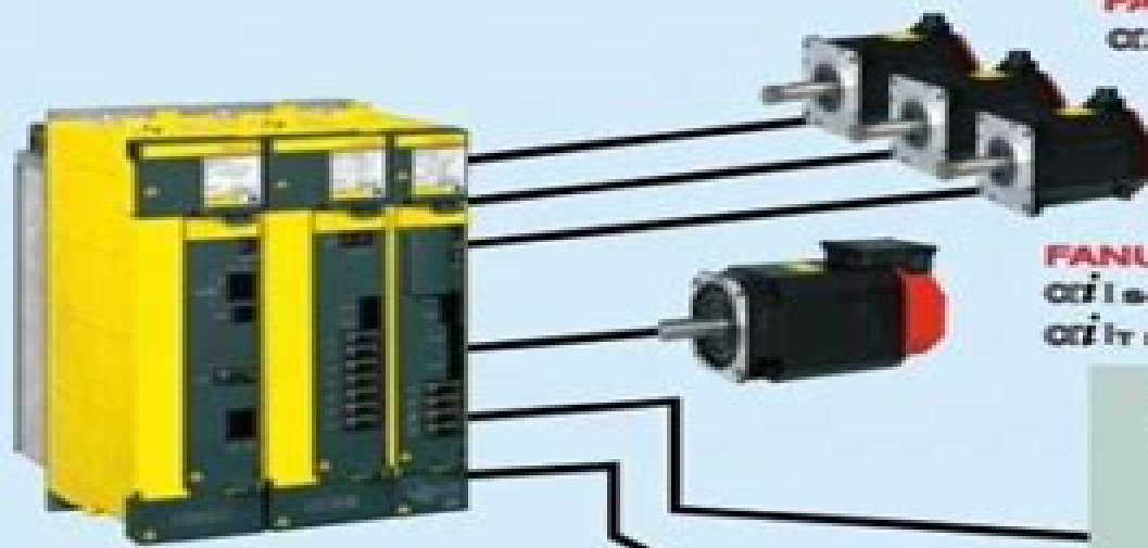
FANUC SERVO AMPLIFIER αiPS series / αiSP series / αiSV series
