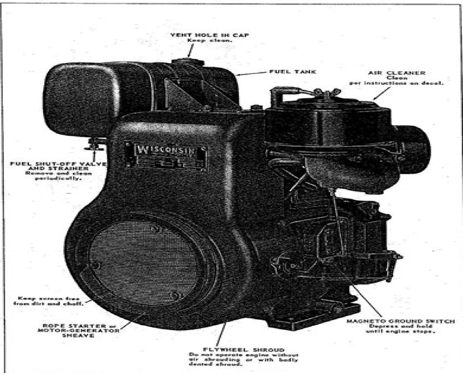
Fig. 2 FAN END (front) and RIGHT HAND SIDE VIEW of ENGINE
