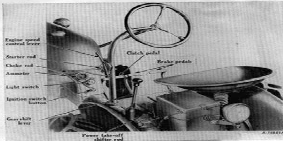
Illustr. 3—Location of Controls.
