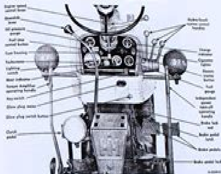
Figure 3 Instruments and controls of the Ford 800 Model Tractor.
