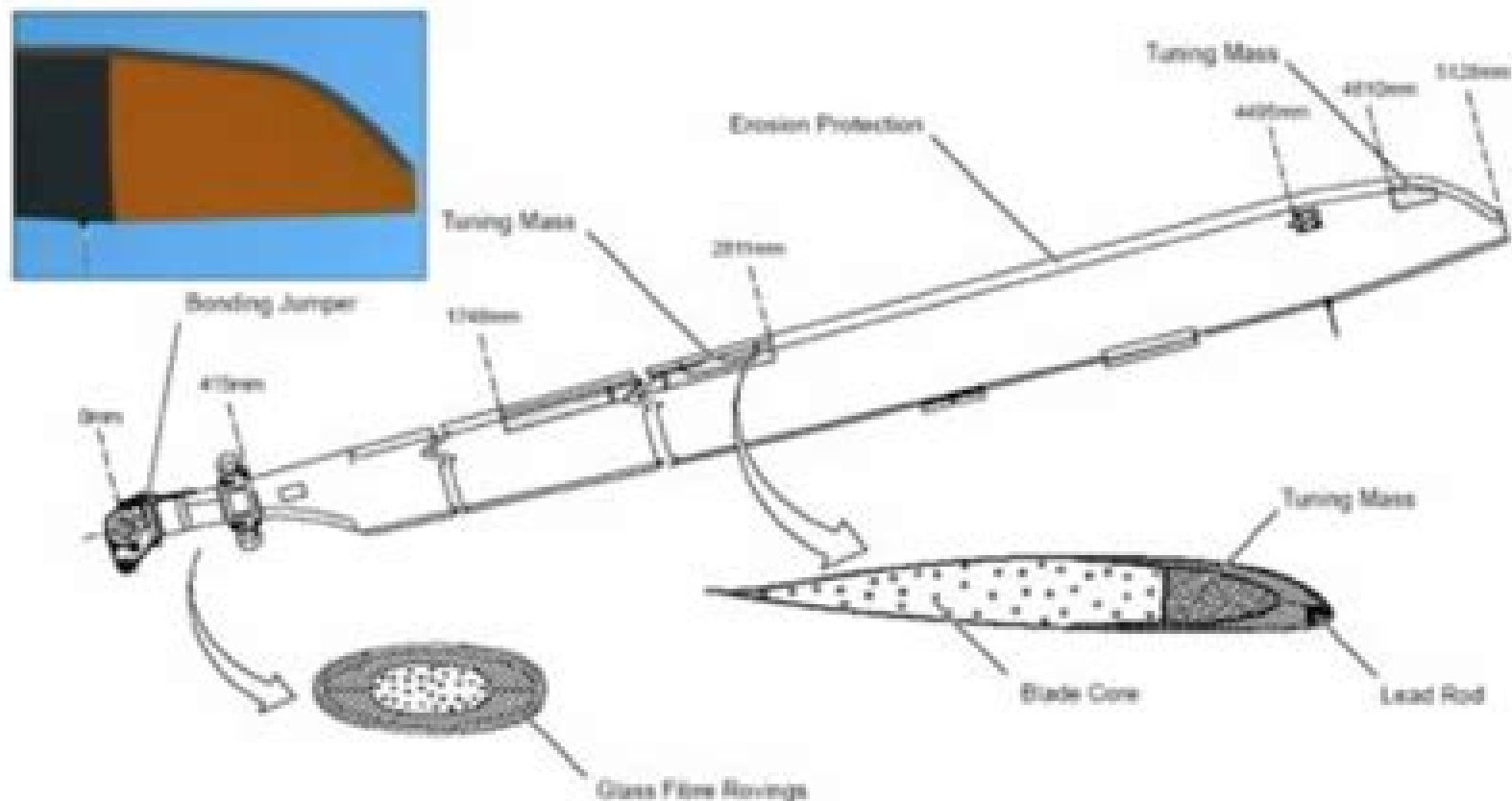
Main Rotor Blade
