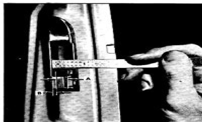
Figure 2-41—Door Lock Striker Engagement
