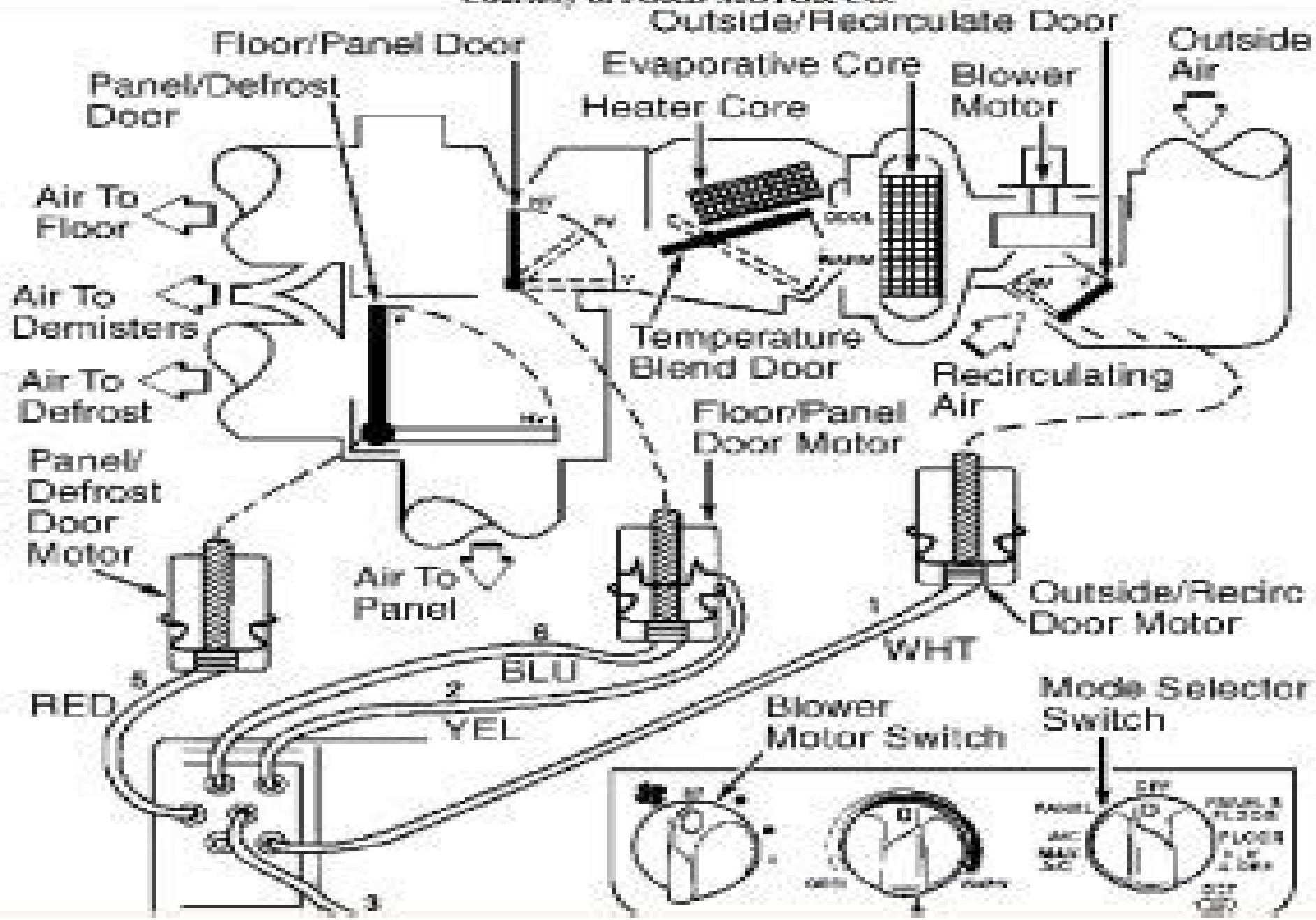
1997 Ford Pickup F150 Fig. 16: Vacuum Schematic Courtesy of FORD MOTOR CO.
