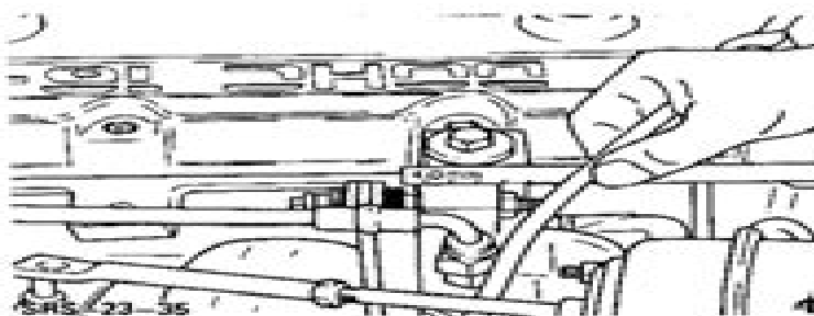
Fig.50. Setting - guide pin shoulder to damper support - 4 mm.
