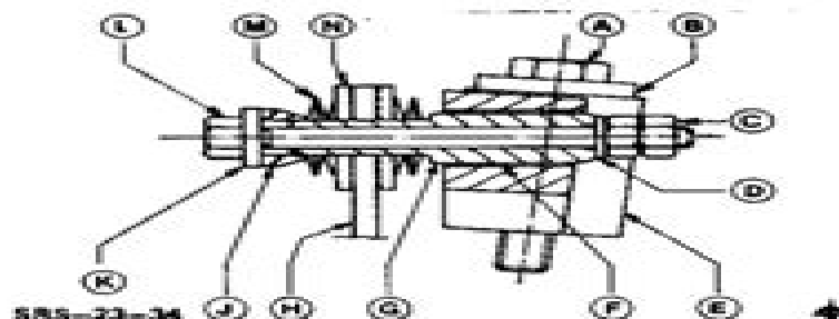
Fig.49. Turbocharger vibration damper cross section.
