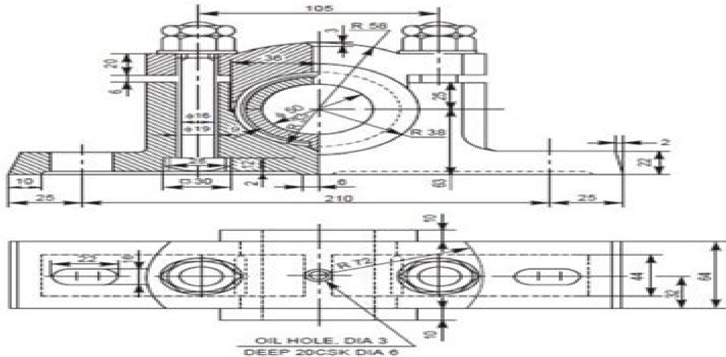
Fig. 12.4 Plummer block
