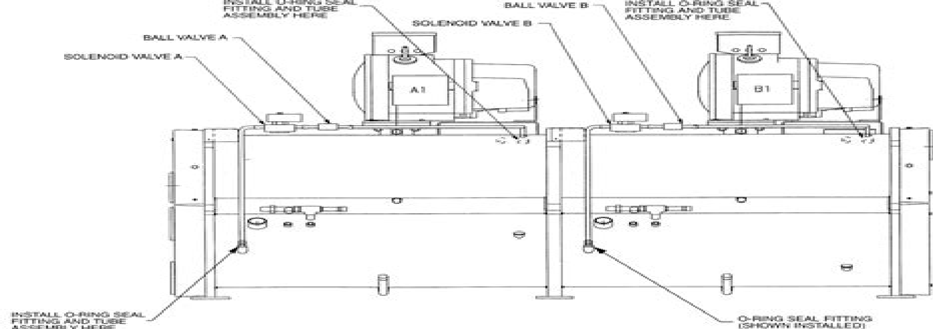
Fig. 2 — Installing Fittings and Valves, 30HX (Typical)
