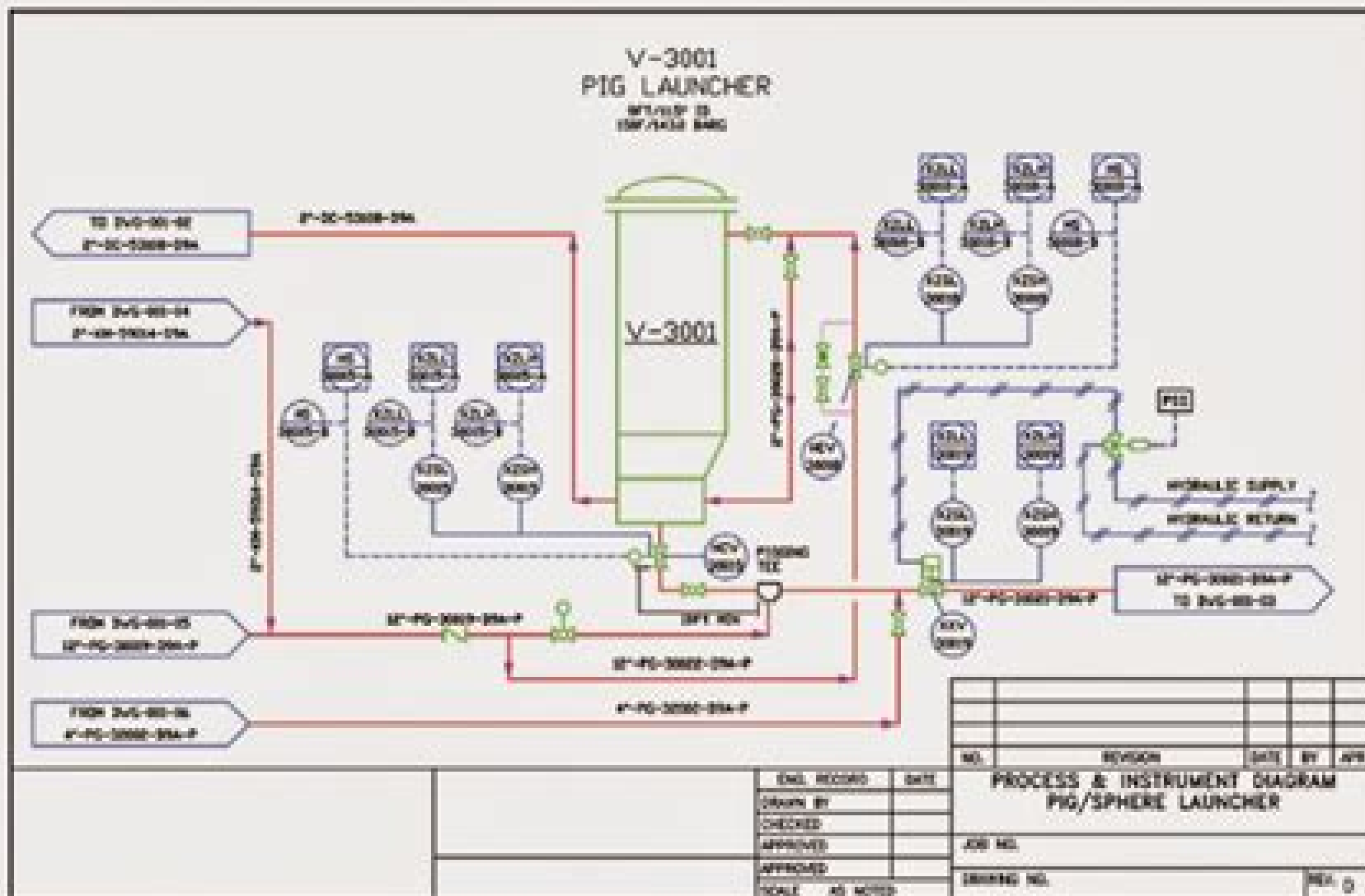
Piping and instrumentation diagram Chemineering.blogspot.com
