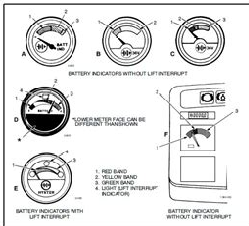
FIGURE 1. BATTERY INDICATORS WITH METER MOVEMENTS
