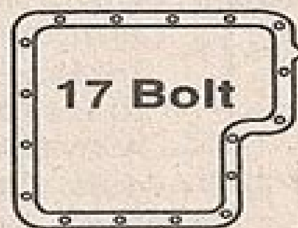
C6 Transmission Tip: The rear edge of the pan is S-shaped.
