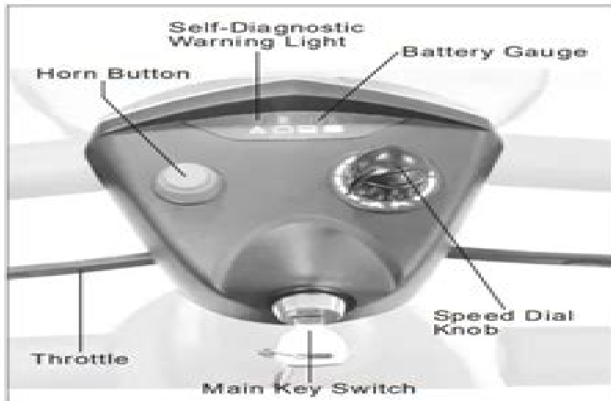
Figure 2 - EW-M39 Top Control Panel
