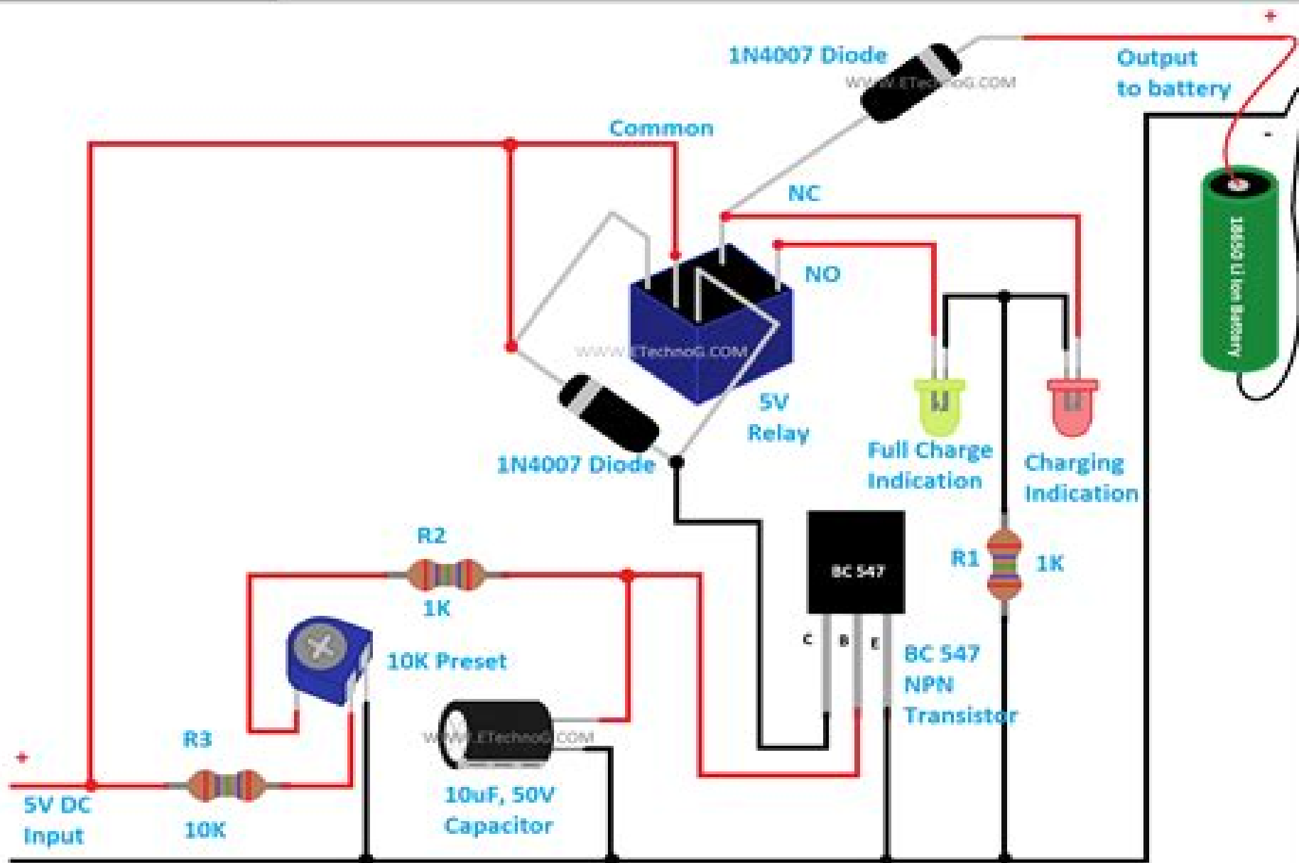
Auto Cutoff 3.7V Lithium Ion Battery Charger Circuit
