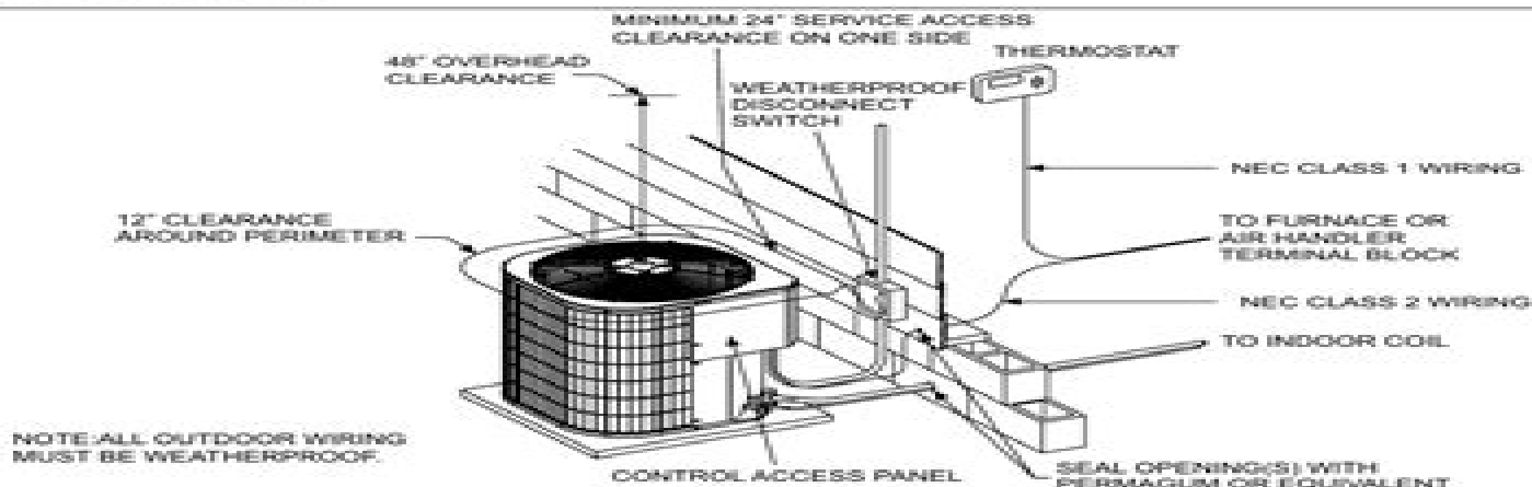
FIGURE 1: Typical Installation
