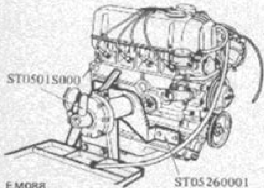
Fig. EM-11 Engine on engine stand
