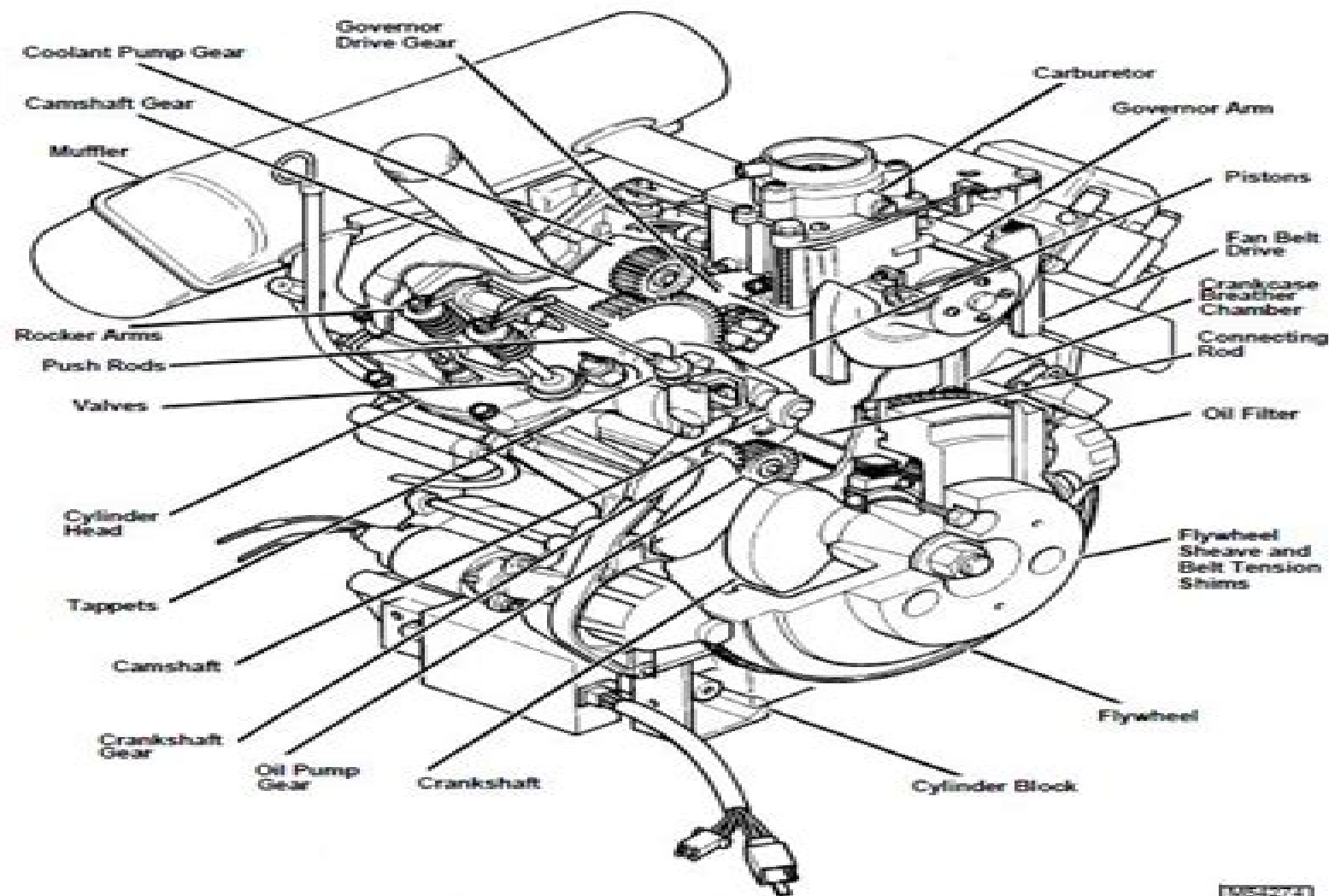
Cutaway—FD620D
