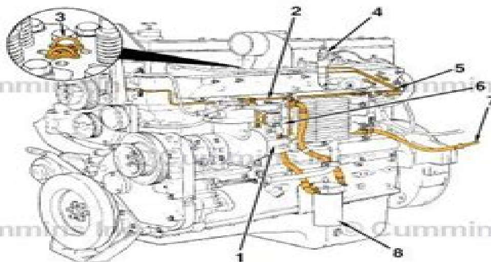
CELECT™ and CELECT™ Plus Fuel System
