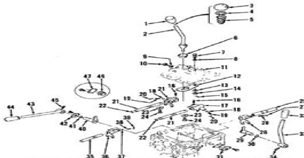
Fig. 79—Exploded view of shifter mechanism used on Models 851000 and 851006. Components 39 through 44 are used on Model 851000 and components 46 and 47 are used on Model 851006.
