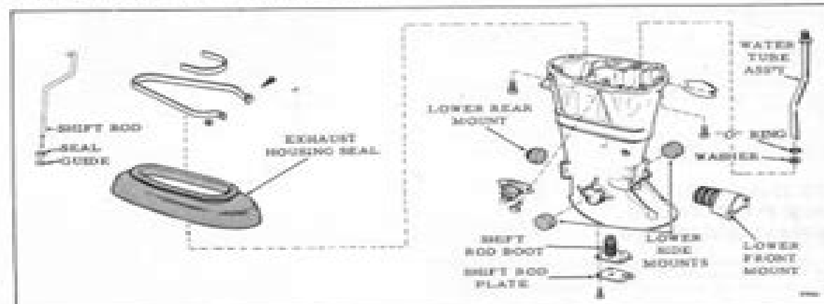
Figure 6-13. Exhaust Housing Assembly View
