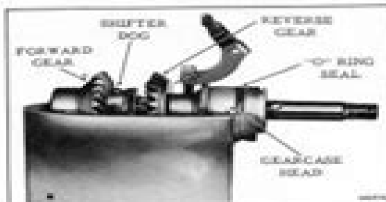
Figure 6-11. Propeller Shaft Assembly
