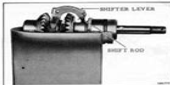
Figure 6-10. Shift Rod Pin and Lever
