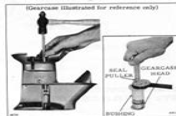
Figure 6-12. Driving Out Shift Rod Seal and Bushing
