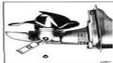
Figure 2-6. Standard Gearcase
