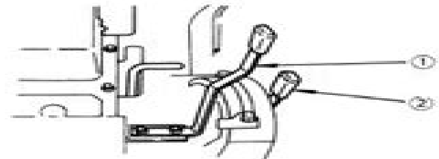
1 - Position control lever 2 - Draft control lever
