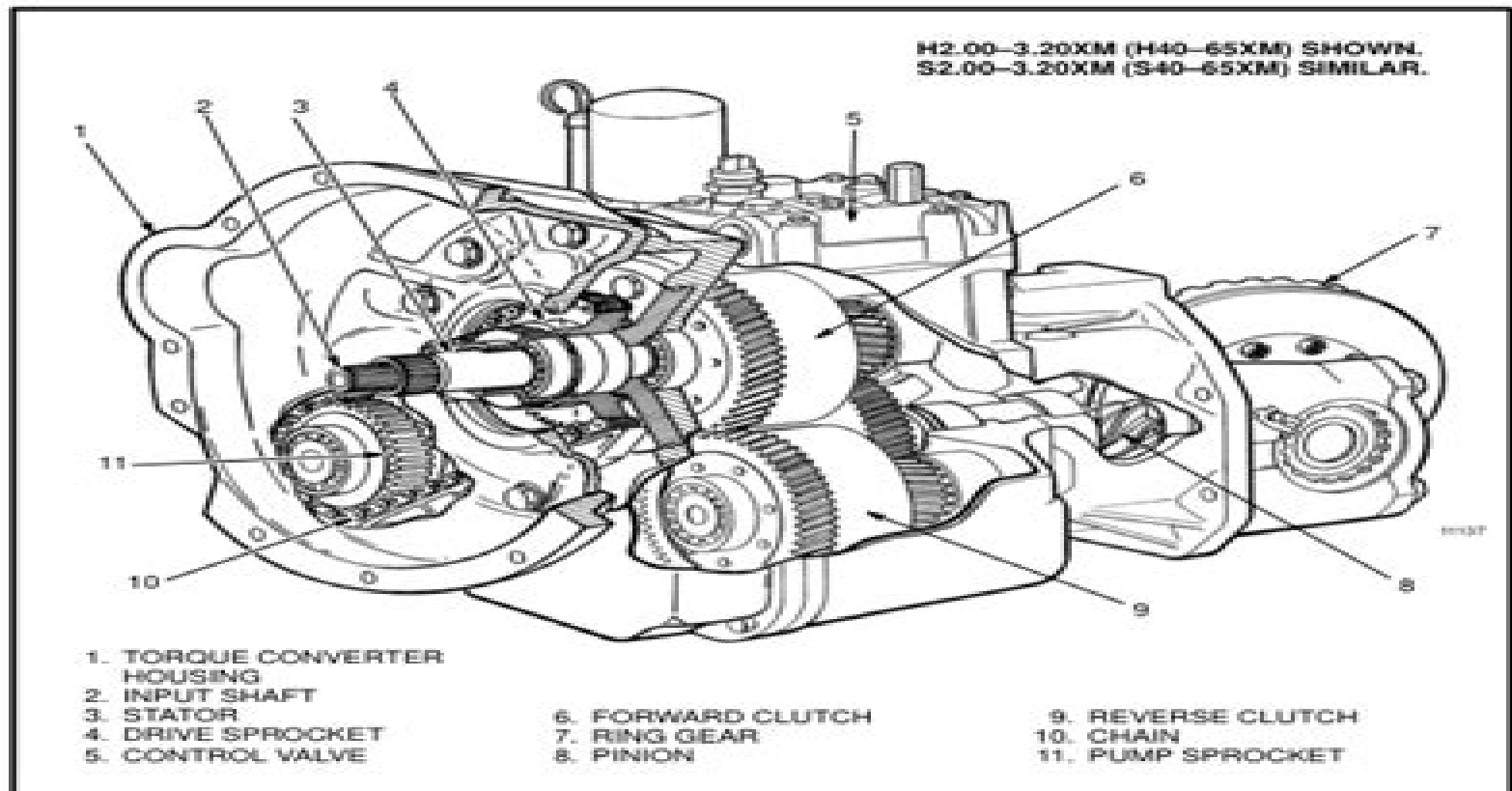
FIGURE 1. TRANSMISSION
