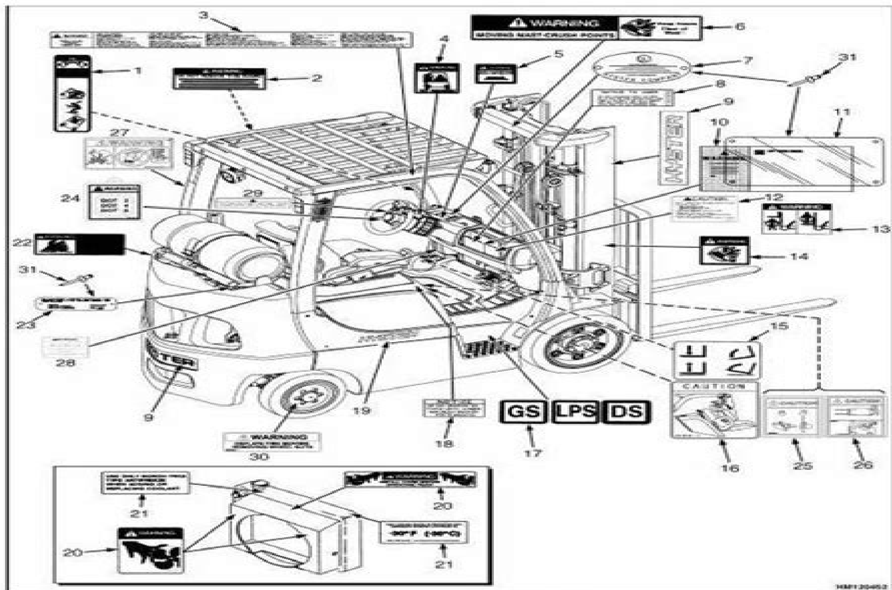
Figure 32. Safety Label Positions
