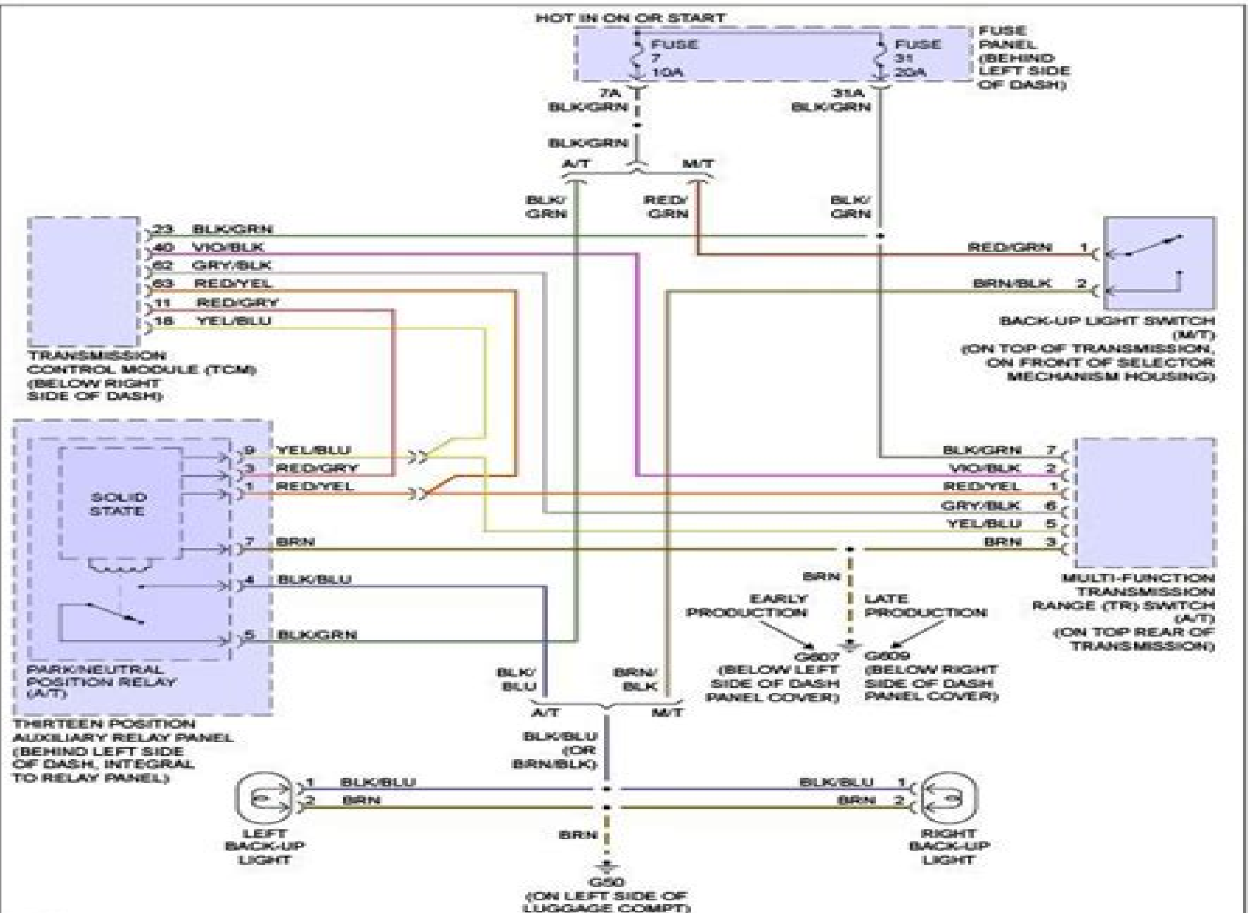
Fig 1: Back-up Lamps Circuit
