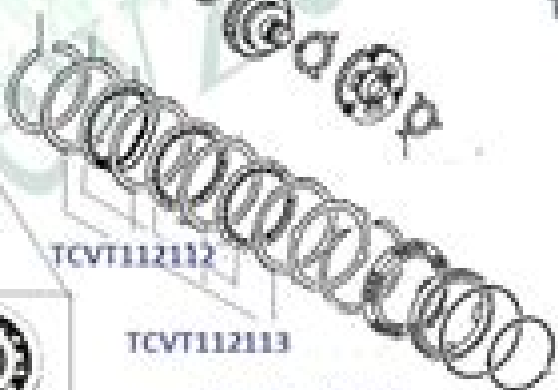
Reverse Clutch
