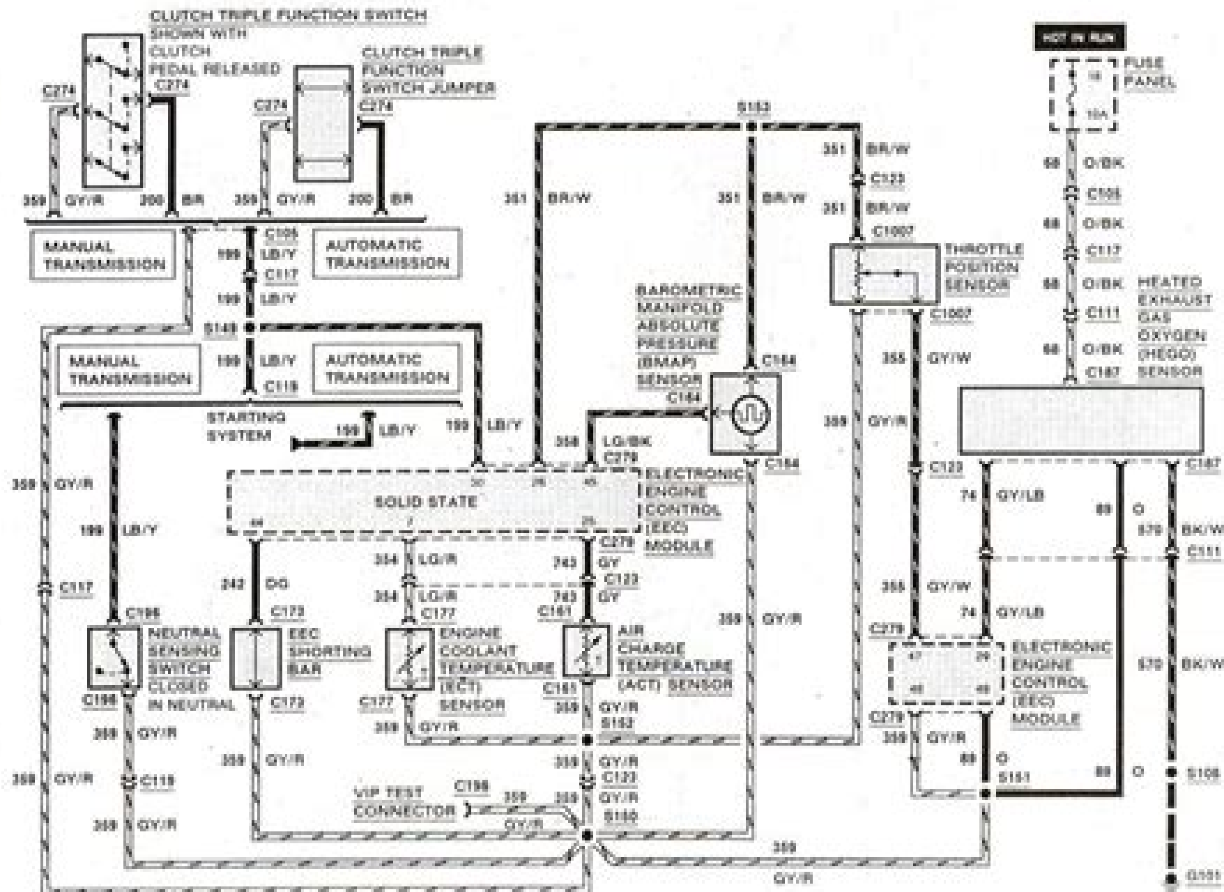
Electronic engine controls, 4.0L engine; 3.0L similar (typical - part 3 of 3)
