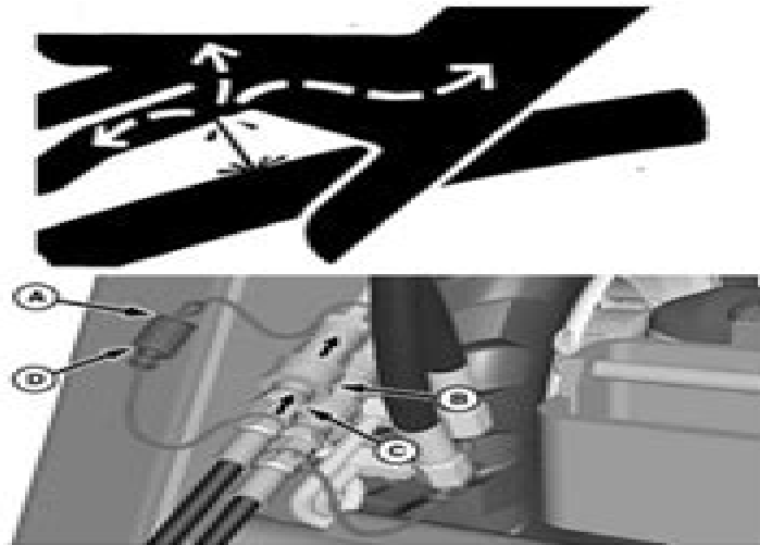
A—Plug (1 per female coupler) B—Coupler, Female (1 per connection) C—Coupler, Male (1 per connection) D—Cap (1 per male coupler)
