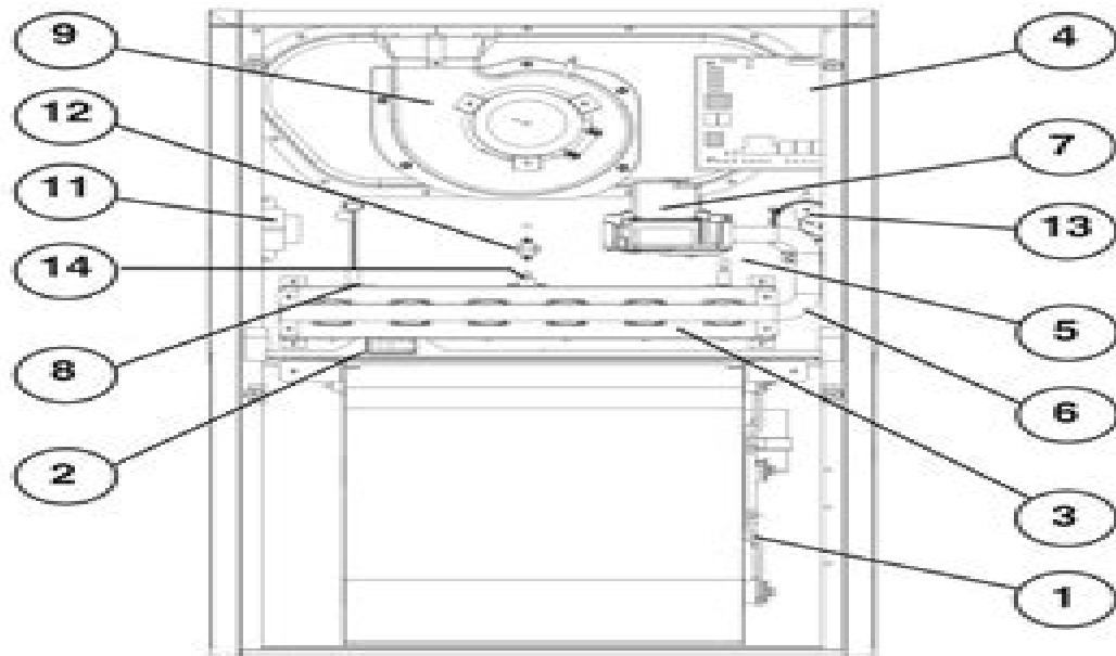
Upflow/Horizontal Gas Furnace
