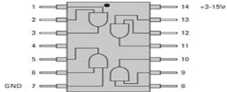
4081 Quad AND
