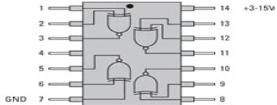
4077 Quad XNOR
