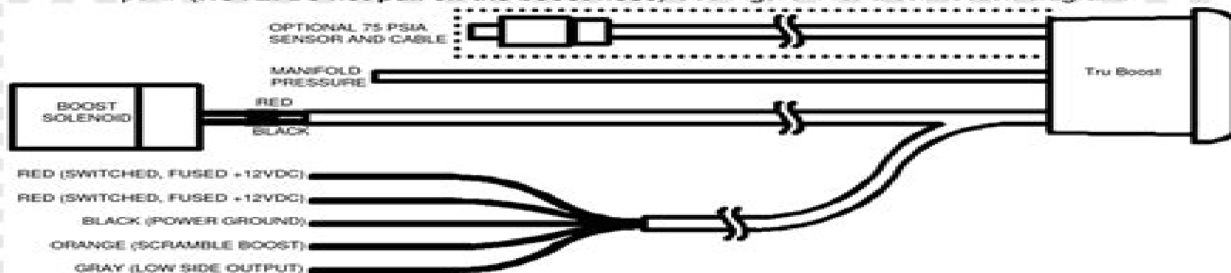
Figure 4. Connection Diagram
