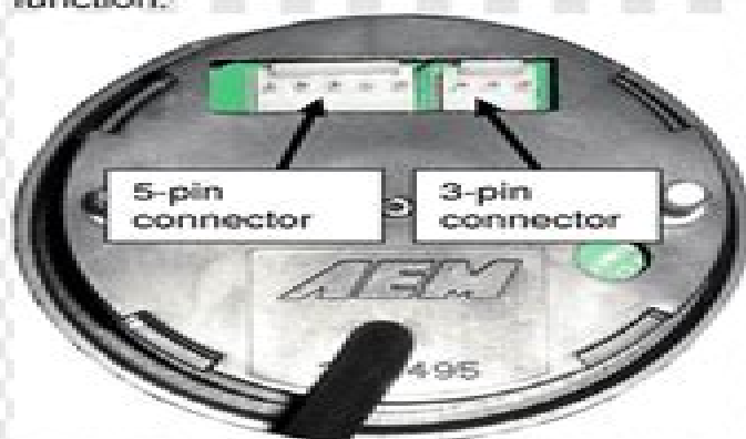
Figure 2. Connector Locations
