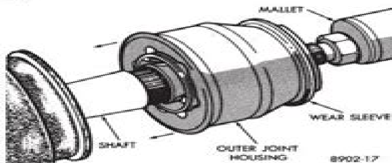
Fig. 21 Joint Installation
