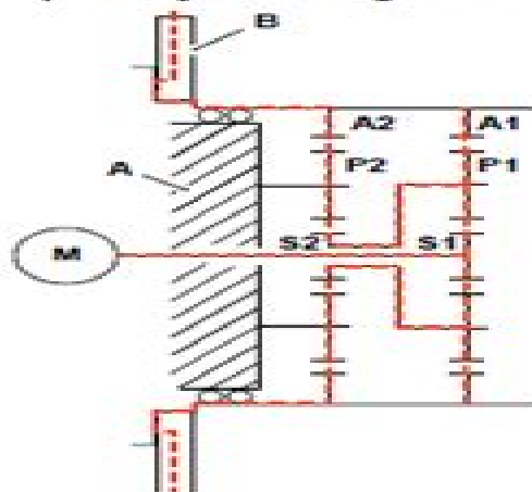
Figure 523. Drive path - two stage planetary reduction gearbox
