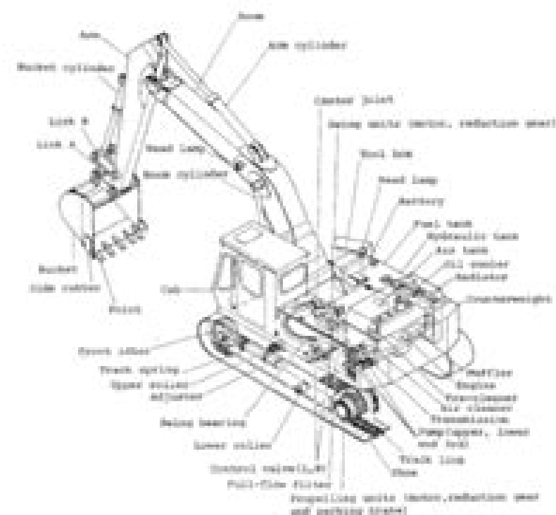
Fig. 2-1 Name of Component Parts
