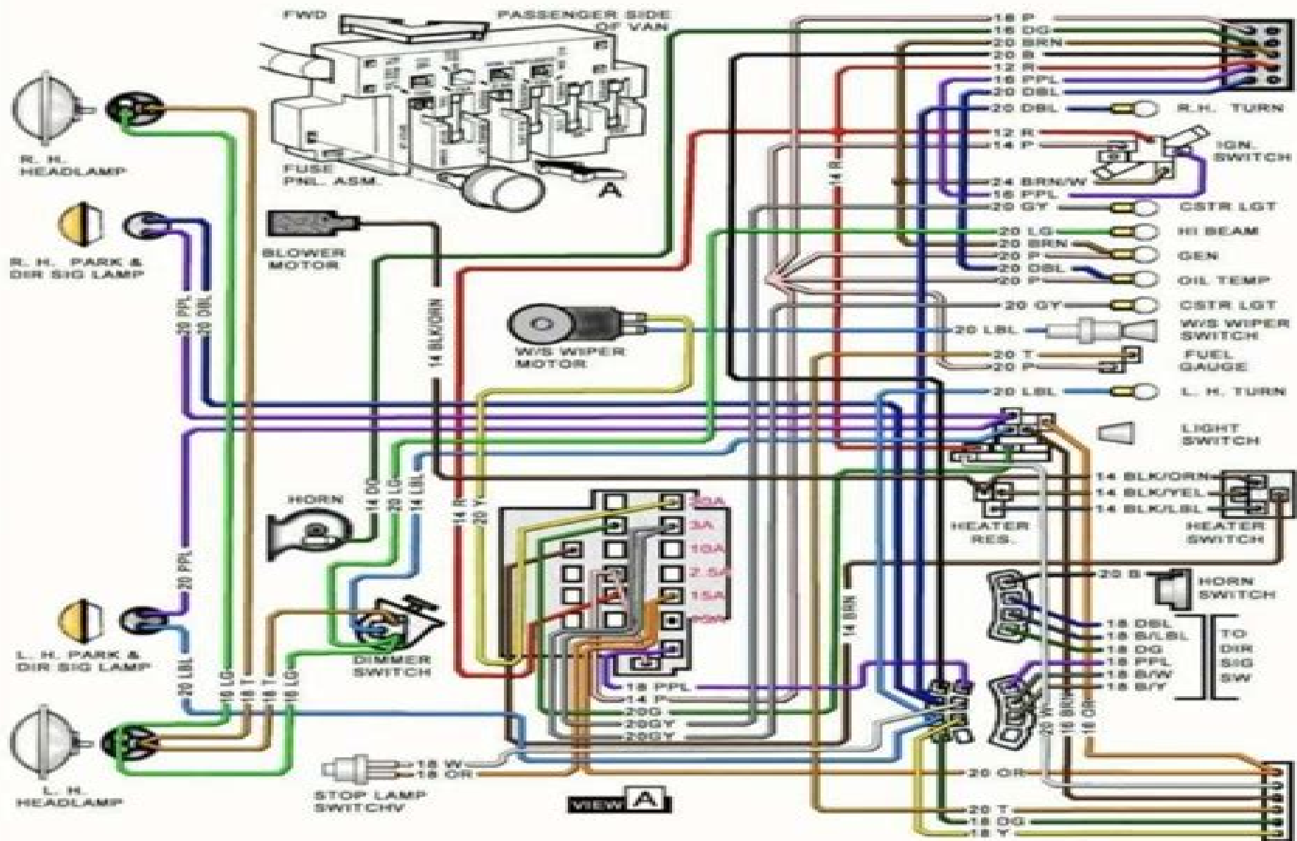
Fig. 43 - Front End & Instrument Panel (1966 Chevy Van)
