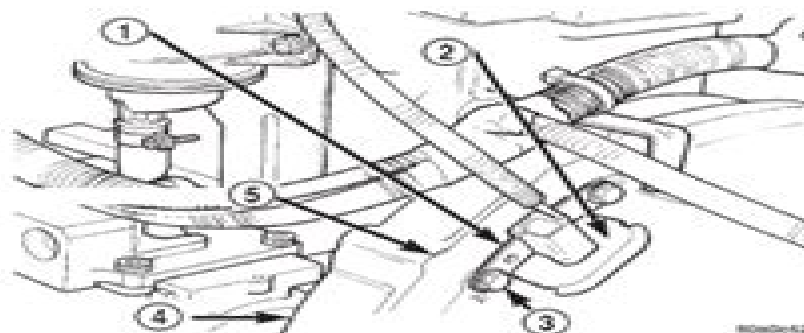
Fig. 21 Engine Speed Sensor
