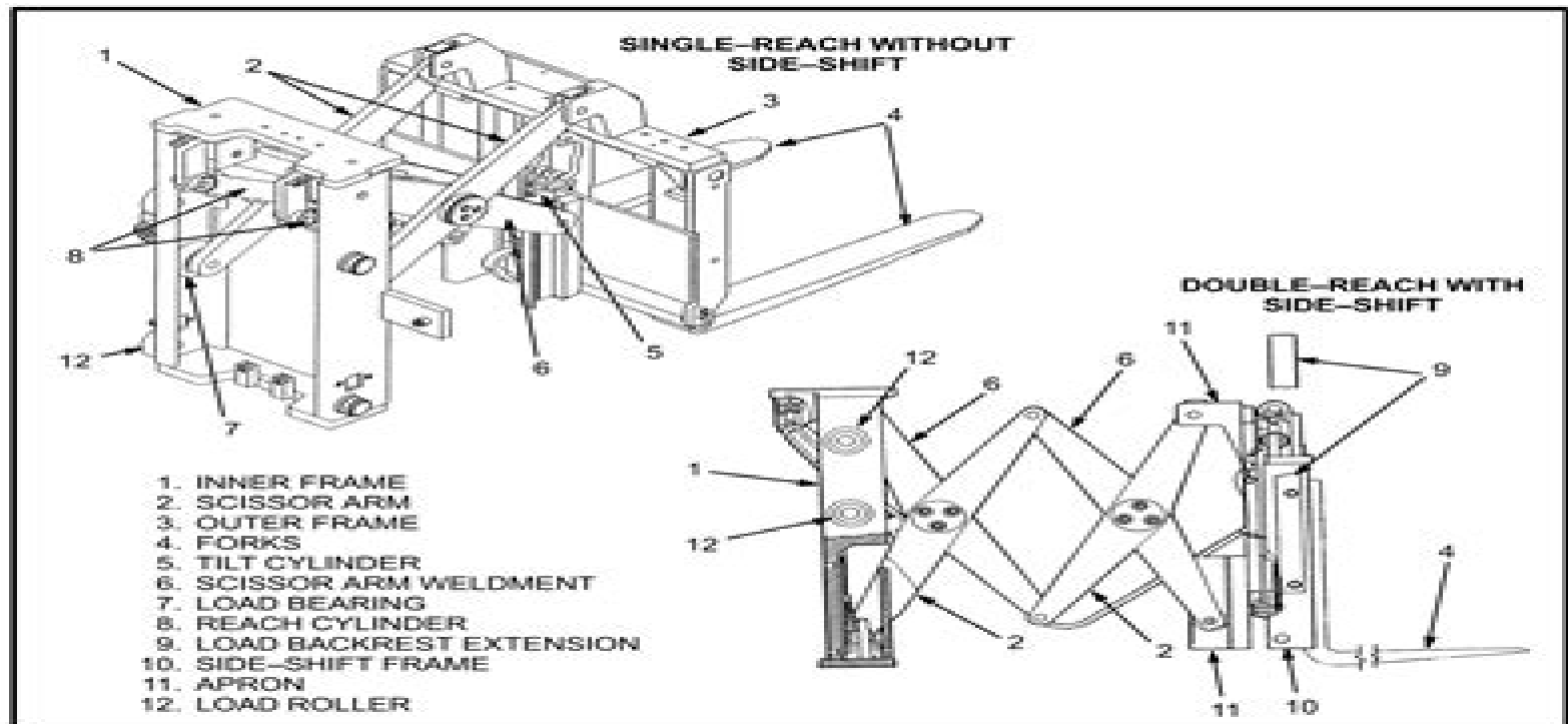
FIGURE 1. REACH CARRIAGES
